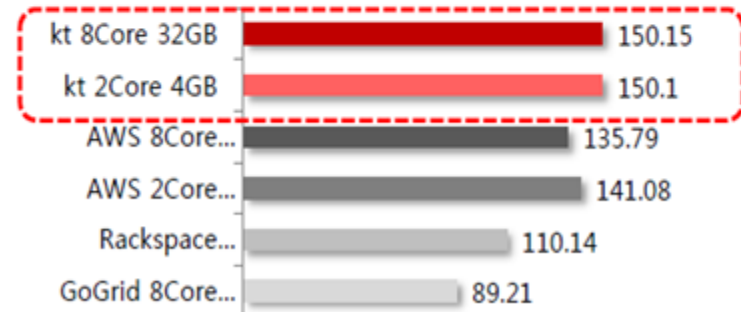
Encoding/Encryption Performance
