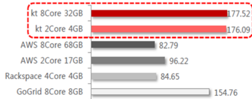
Encoding/Encryption Performance
